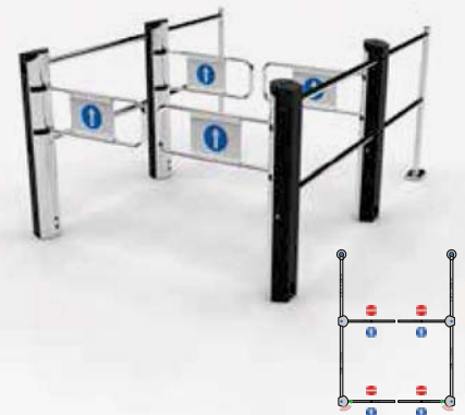
Easygate NG PEC/Radar (first pair) & Easygate NG Standard (second pair). Double saloon with lead out rails. Opening is controlled by built-in radar (first gate pair) and photo-electric cell (second gate pair).
